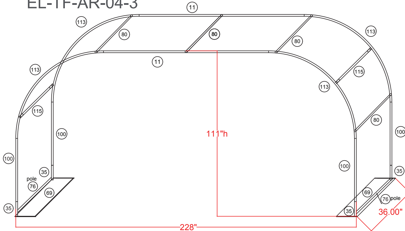
36"d x 228"w x 111"h Curved Arch Display
