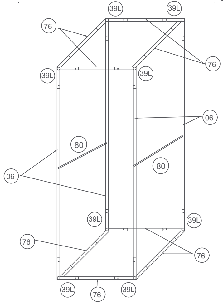
Isometric View
